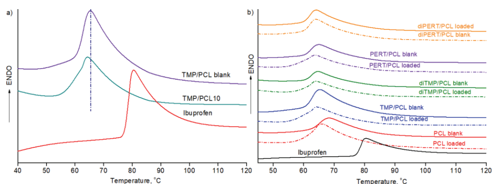
Fig. 2. DSC thermograms of: a) TmPCL microspheres and IB, and b) all microspheres.
