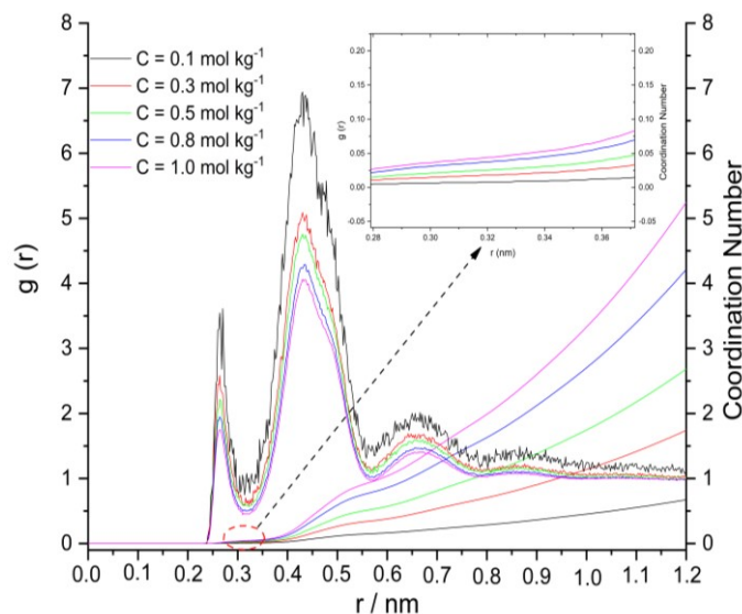
Fig 3. Radial distribution functions \{g_{K-F}(r)\} at various concentrations
