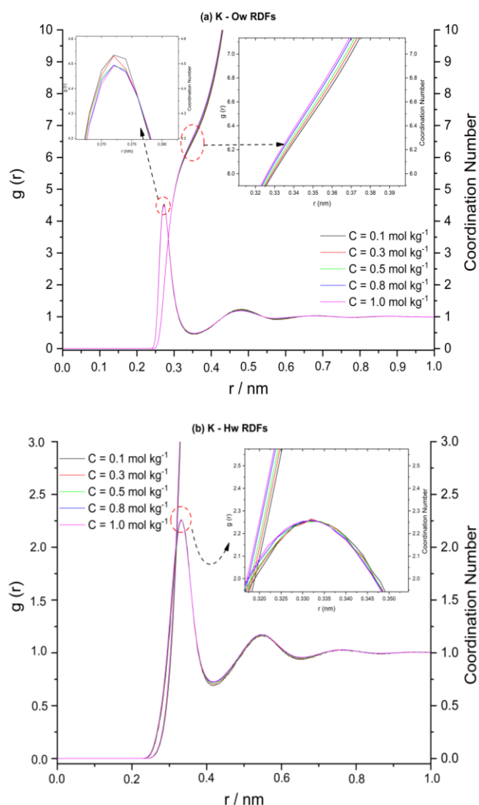
Fig 1. g_{\text{K-Ow}}(r) and g_{\text{K-Hw}}(r) for potassium cation at various concentrations.
