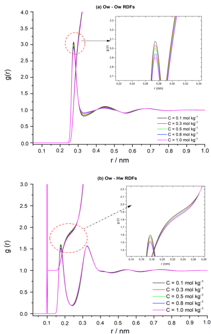
Fig 4. g_{Ow-Ow}(r) and g_{Ow-Hw}(r) functions at various concentrations.
