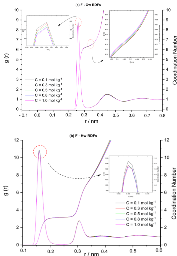
Fig 2. g_{\text{F-Ow}}(r) and g_{\text{F-Hw}}(r) for fluoride anion at various concentrations.
