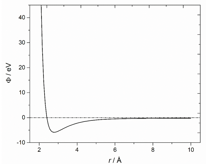
Fig. S-2. The U-N interaction potential represented by formula (S1).
