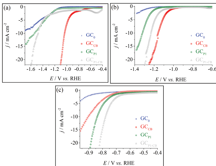
Fig. 3. Cathodic polarization curves recorded on \text{GC}_0 , \text{GC}_{\text{CB}} , \text{GC}_{\text{PI}} and \text{GC}_{\text{PI-CB}} in the following electrolyte solutions: a) 0.1 \text{ mol L}^{-1} \text{ H}_2\text{SO}_4 , b) 0.1 \text{ mol L}^{-1} \text{ KCl} and c) 1 \text{ mol L}^{-1} \text{ KOH} . \nu = 5 \text{ mV s}^{-1} .
