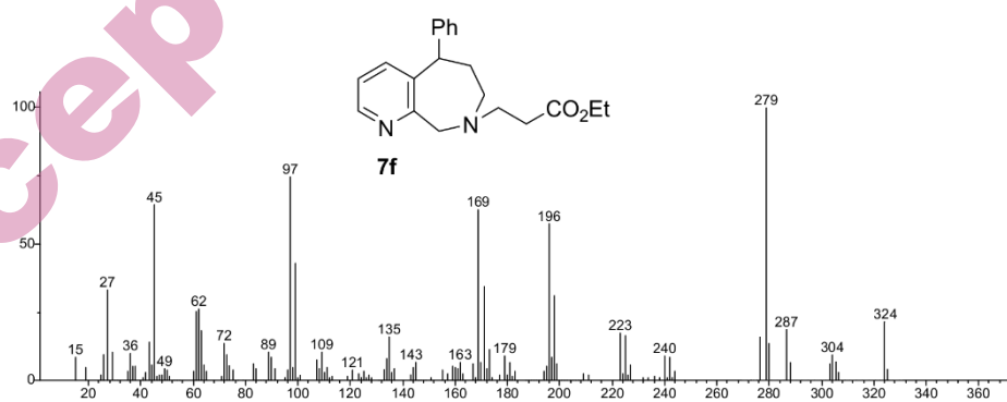
Fig. S-42. Mass spectrum of compound 7f
