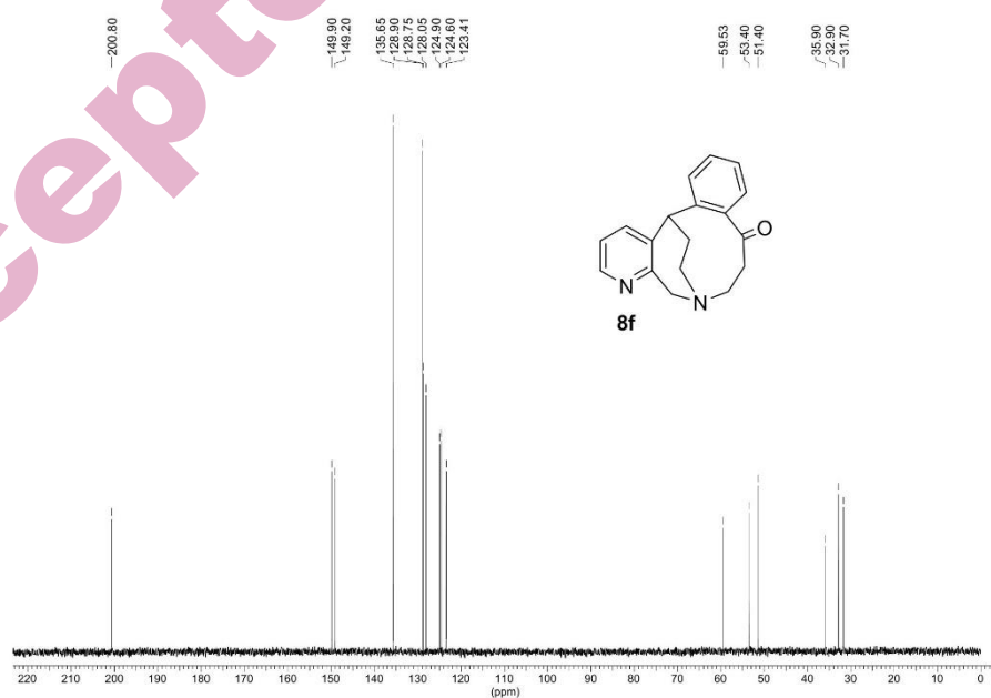
Fig. S-56. 13 C-NMR spectrum of compound 8f
