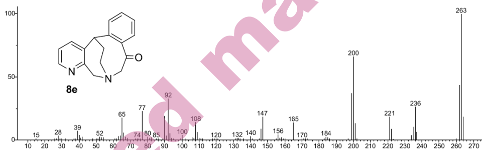
Fig. S-65. Mass spectrum of compound 8e
