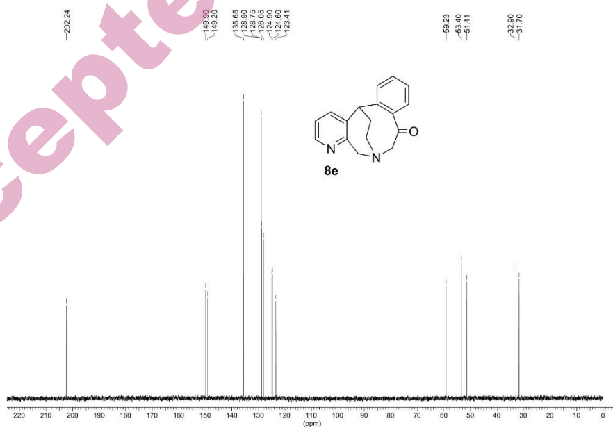
Fig. S-54. 13 C-NMR spectrum of compound 8e
