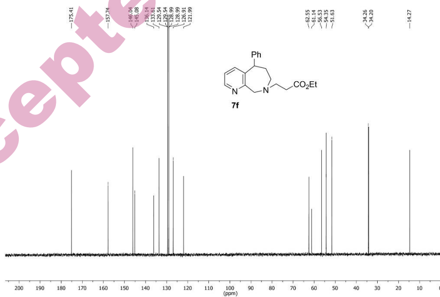
Fig. S-20. 13 C-NMR spectrum of compound 7f
