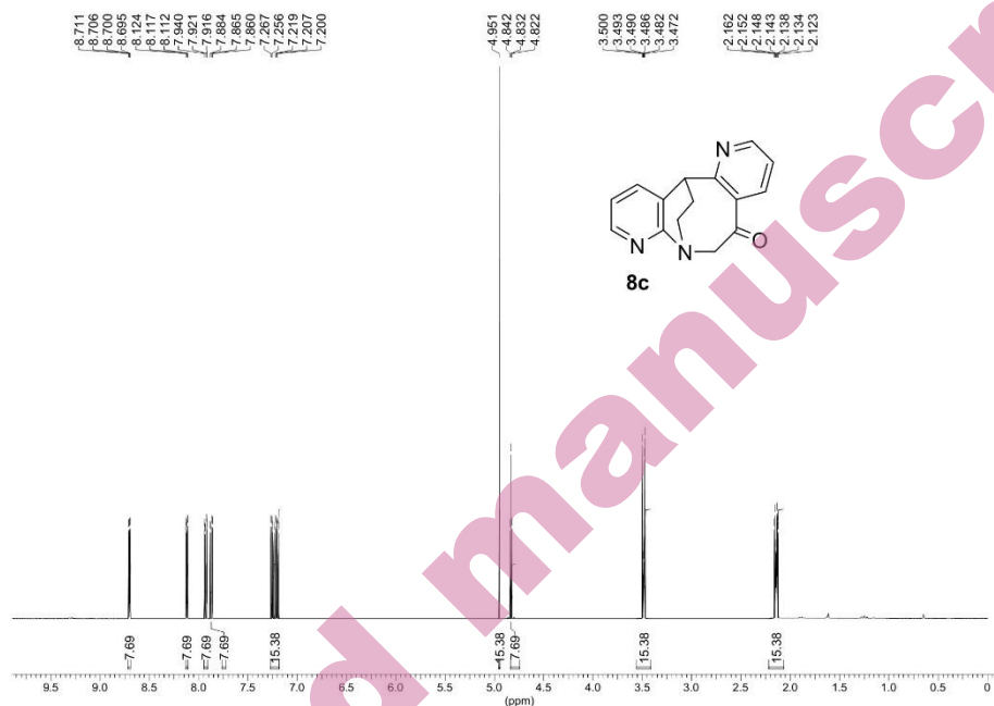
Fig. S-49. 1 H-NMR spectrum of compound 8c
