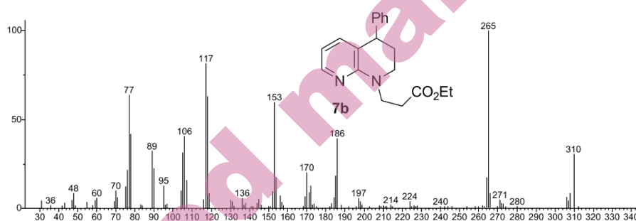
Fig. S-38. Mass spectrum of compound 7b
