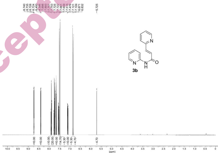
Fig. S-2. 1 H-NMR spectrum of compound 3b
