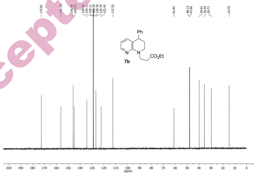
Fig. S-12. 13 C-NMR spectrum of compound 7b
