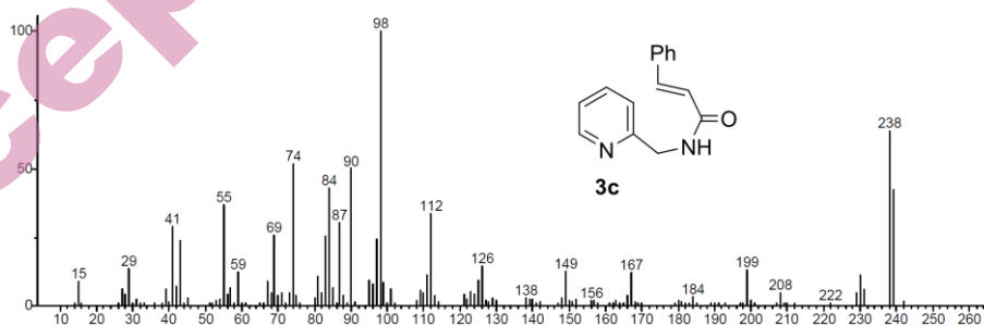
Fig. S-27. Mass spectrum of compound 3c
