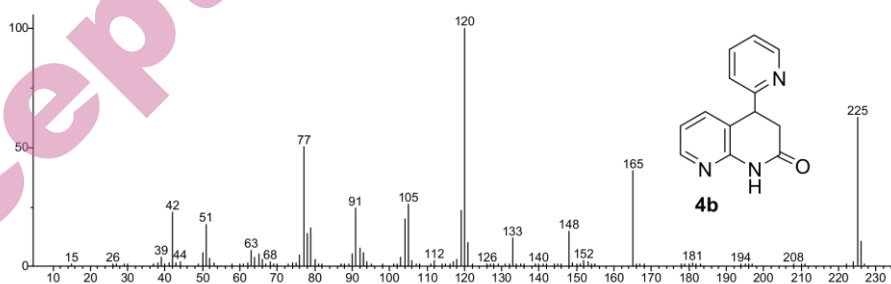
Fig. S-30. Mass spectrum of compound 4b
