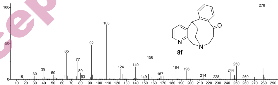
Fig. S-66. Mass spectrum of compound 8f
