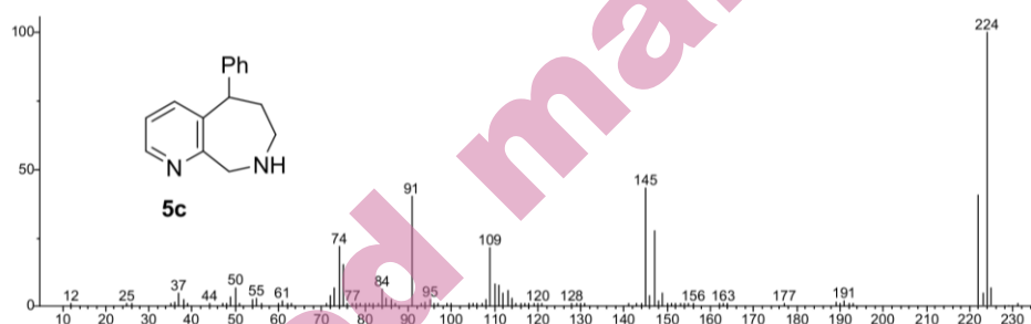
Fig. S-35. Mass spectrum of compound 5c
