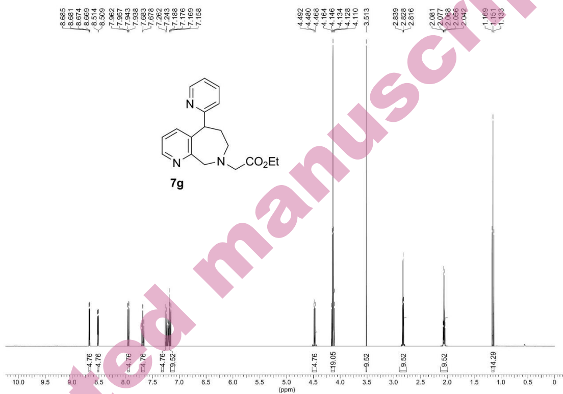
Fig. S-21. 1 H-NMR spectrum of compound 7g
