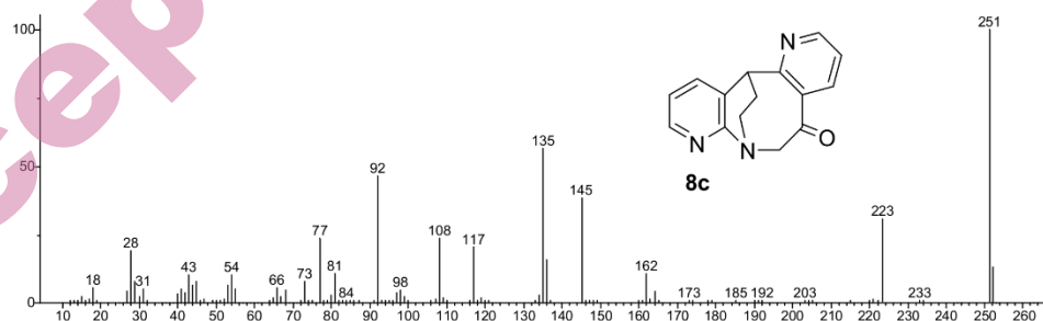
Fig. S-63. Mass spectrum of compound 8c
