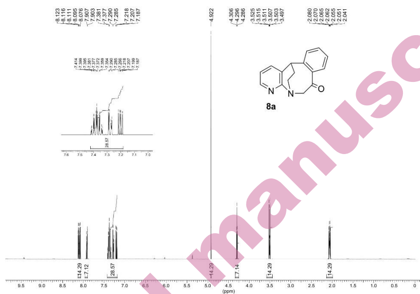
Fig. S-45. 1 H-NMR spectrum of compound 8a
