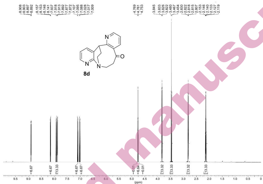
Fig. S-51. 1 H-NMR spectrum of compound 8d
