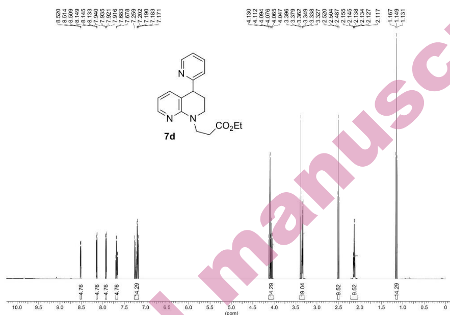
Fig. S-15. 1 H-NMR spectrum of compound 7d
