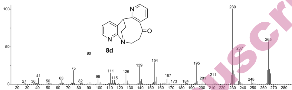
Fig. S-64. Mass spectrum of compound 8d
