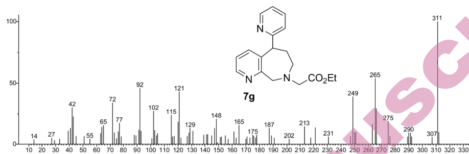
Fig. S-43. Mass spectrum of compound 7g
