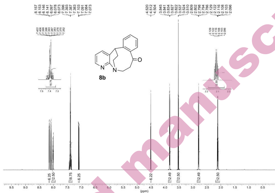
Fig. S-47. 1 H-NMR spectrum of compound 8b
