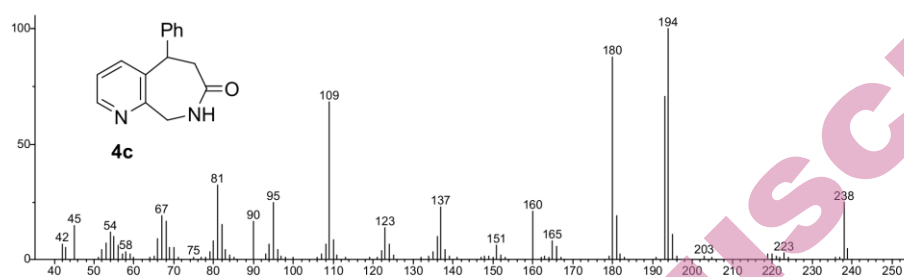
Fig. S-31. Mass spectrum of compound 4c
