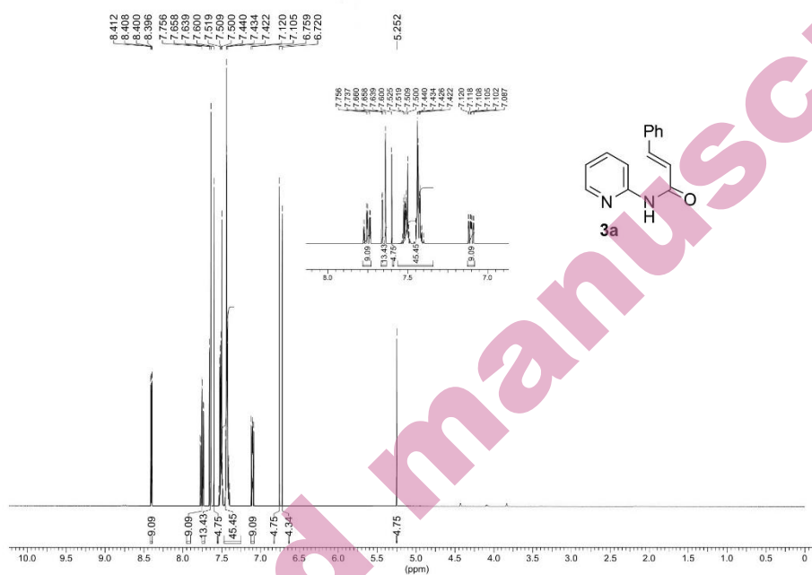
Fig. S-1. 1 H-NMR spectrum of compound 3a
