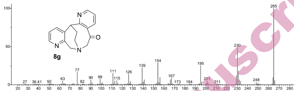
Fig. S-67. Mass spectrum of compound 8g
