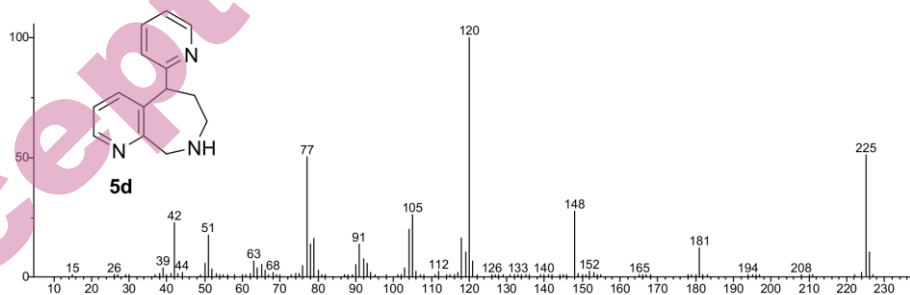
Fig. S-36. Mass spectrum of compound 5d
