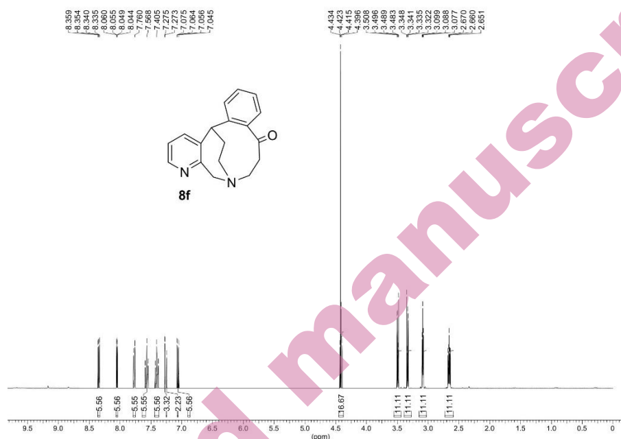
Fig. S-55. 1 H-NMR spectrum of compound 8f
