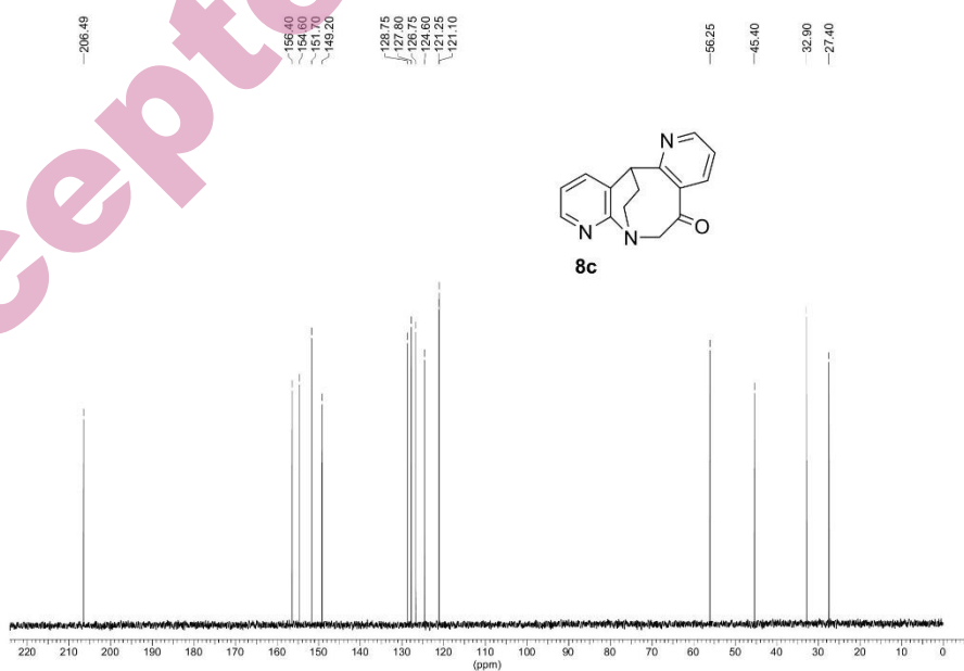
Fig. S-50. 13 C-NMR spectrum of compound 8c
