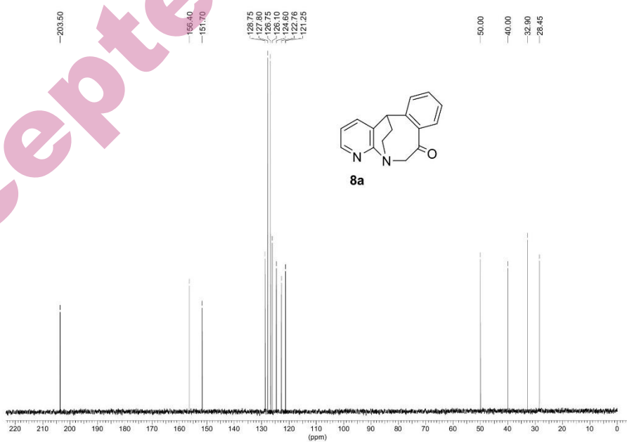
Fig. S-46. 13 C-NMR spectrum of compound 8a
