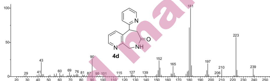
Fig. S-32. Mass spectrum of compound 4d
