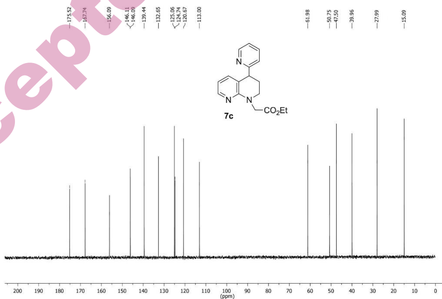
Fig. S-14. 13 C-NMR spectrum of compound 7c
