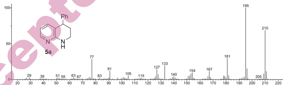
Fig. S-33. Mass spectrum of compound 5a
