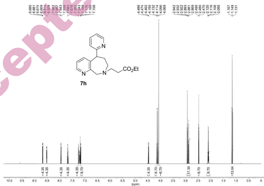
Fig. S-23. 1 H-NMR spectrum of compound 7h
