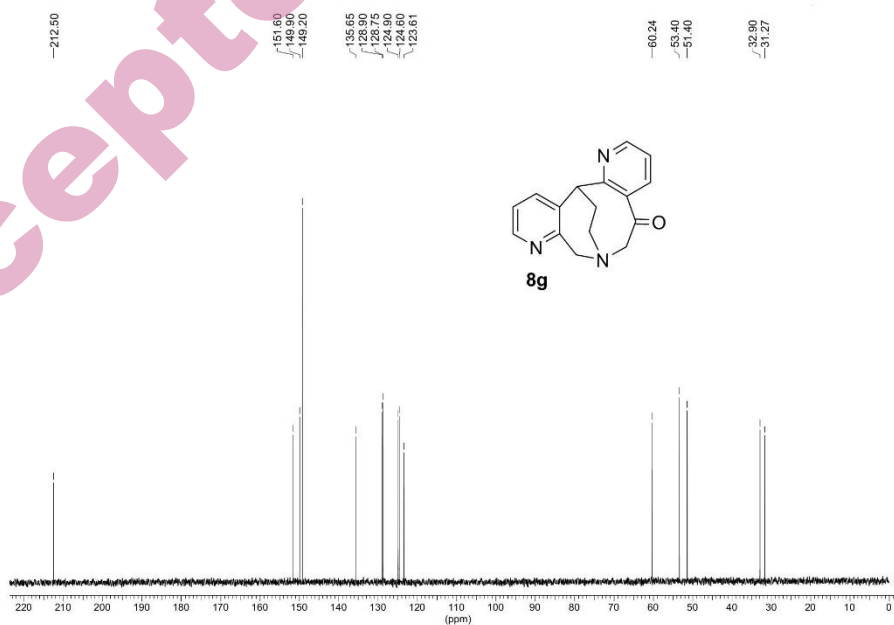
Fig. S-58. 13 C-NMR spectrum of compound 8g
