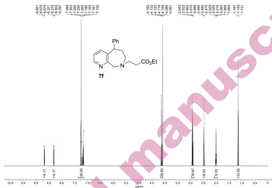
Fig. S-19. 1 H-NMR spectrum of compound 7f
