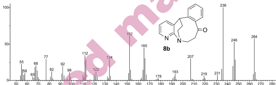
Fig. S-62. Mass spectrum of compound 8b
