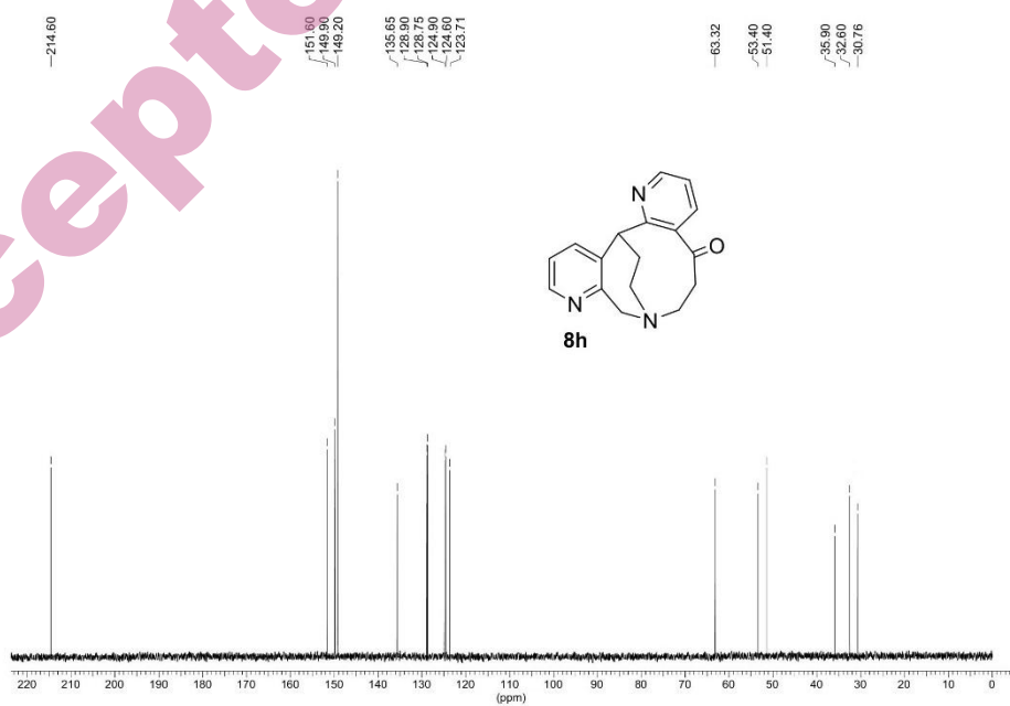
Fig. S-60. 13 C-NMR spectrum of compound 8h
