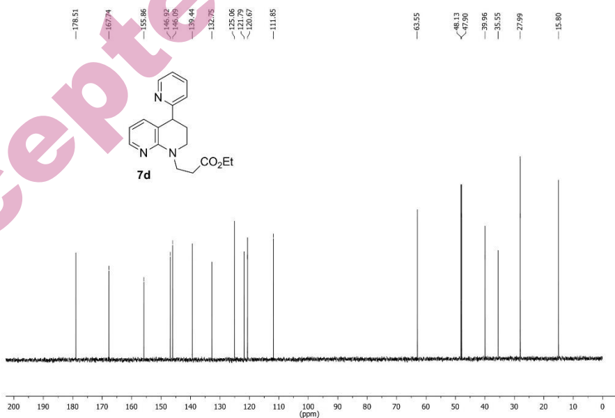
Fig. S-16. 13 C-NMR spectrum of compound 7d
