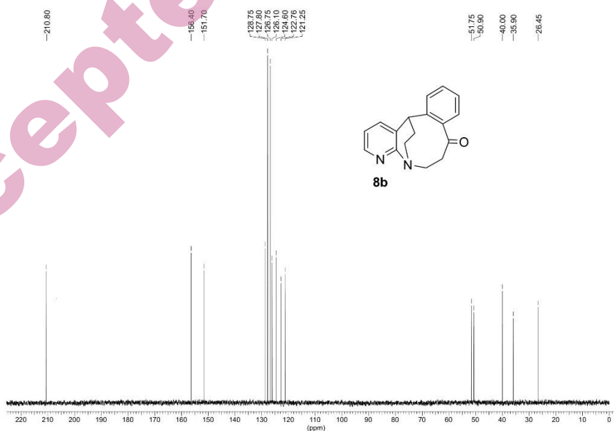
Fig. S-48. 13 C-NMR spectrum of compound 8b
