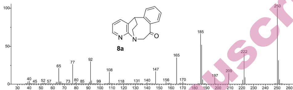
Fig. S-61. Mass spectrum of compound 8a
