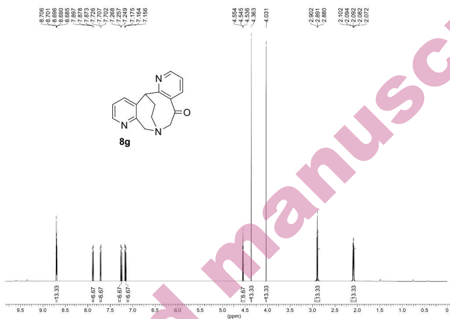
Fig. S-57. 1 H-NMR spectrum of compound 8g
